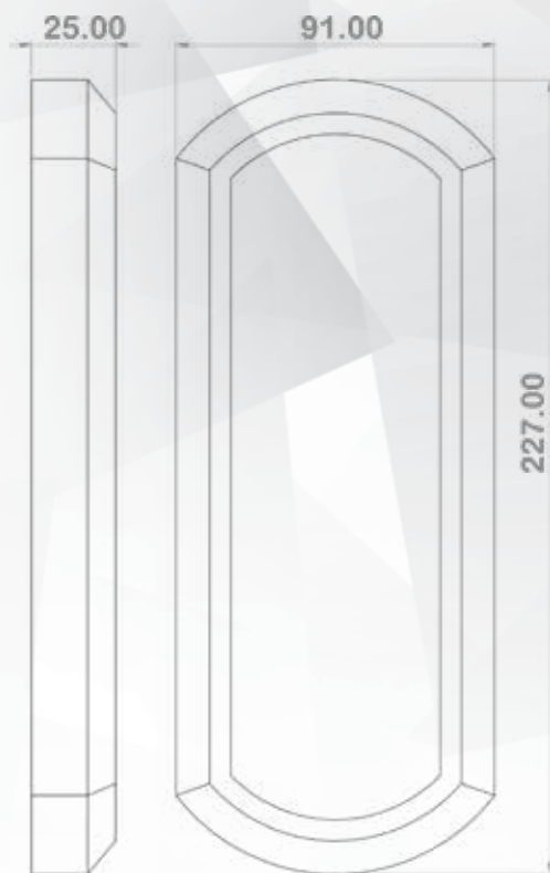
FS - PLAN (mm)
