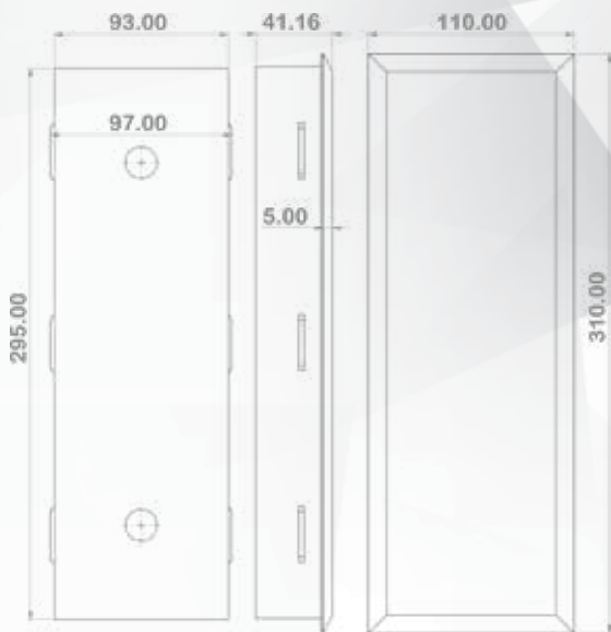
FG11P - PLAN (mm)
