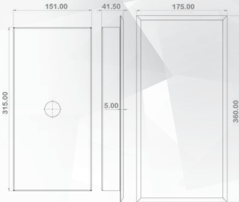
FGD - PLAN (mm)
